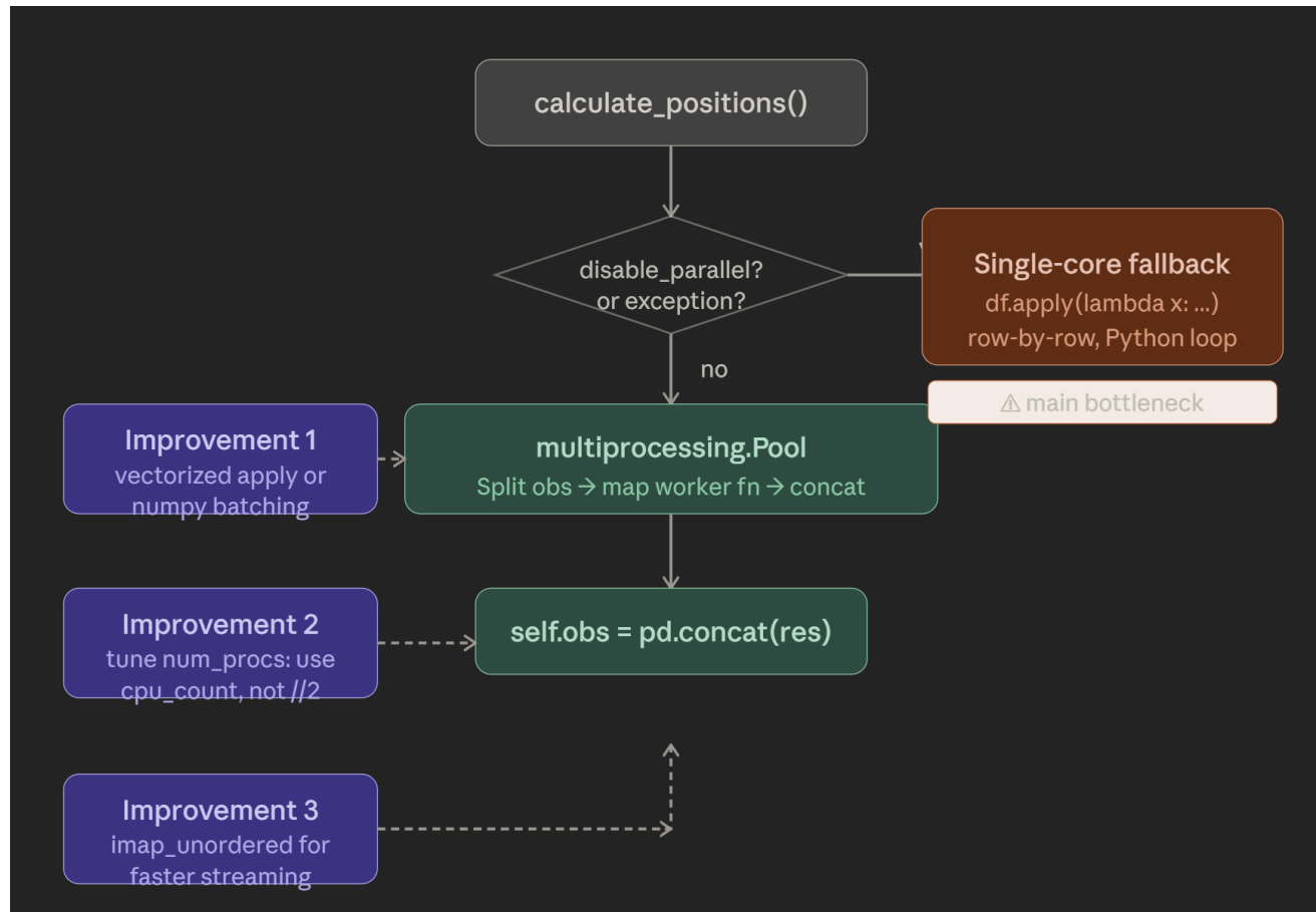
Flowchart with potential improvements for calculate_positions()
